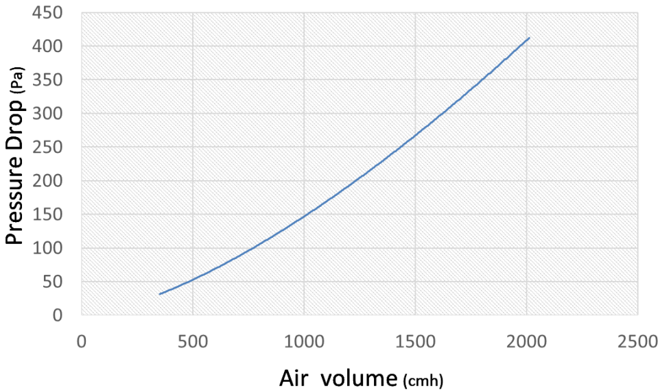
<Pressure drop >
